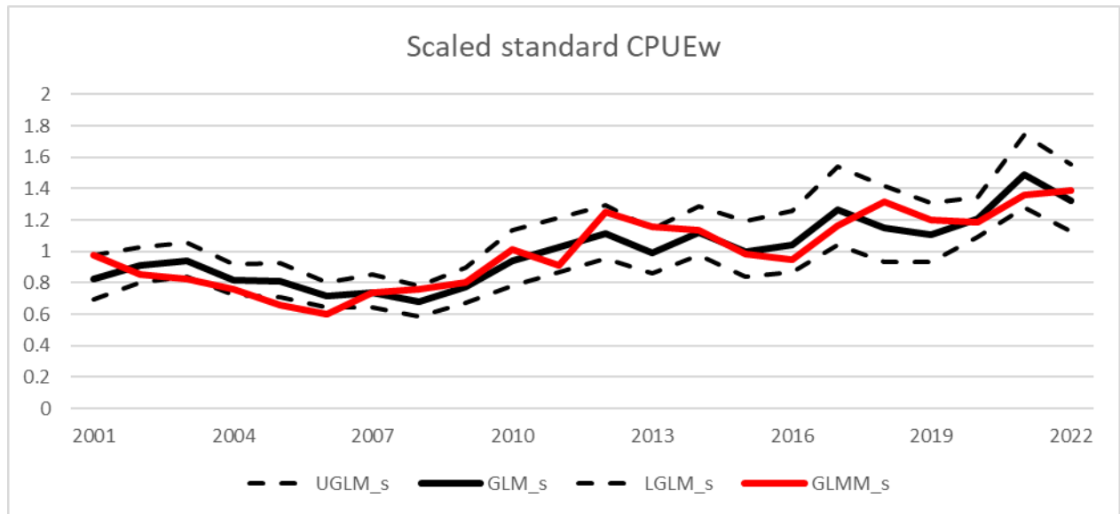
Figure 6. Comparative scaled standardized CPUE in weight, GLM versus GLMM (MIXED), obtained in the Indian Ocean for the period 2001-2022. Both series are scaled from their respective mean value.
