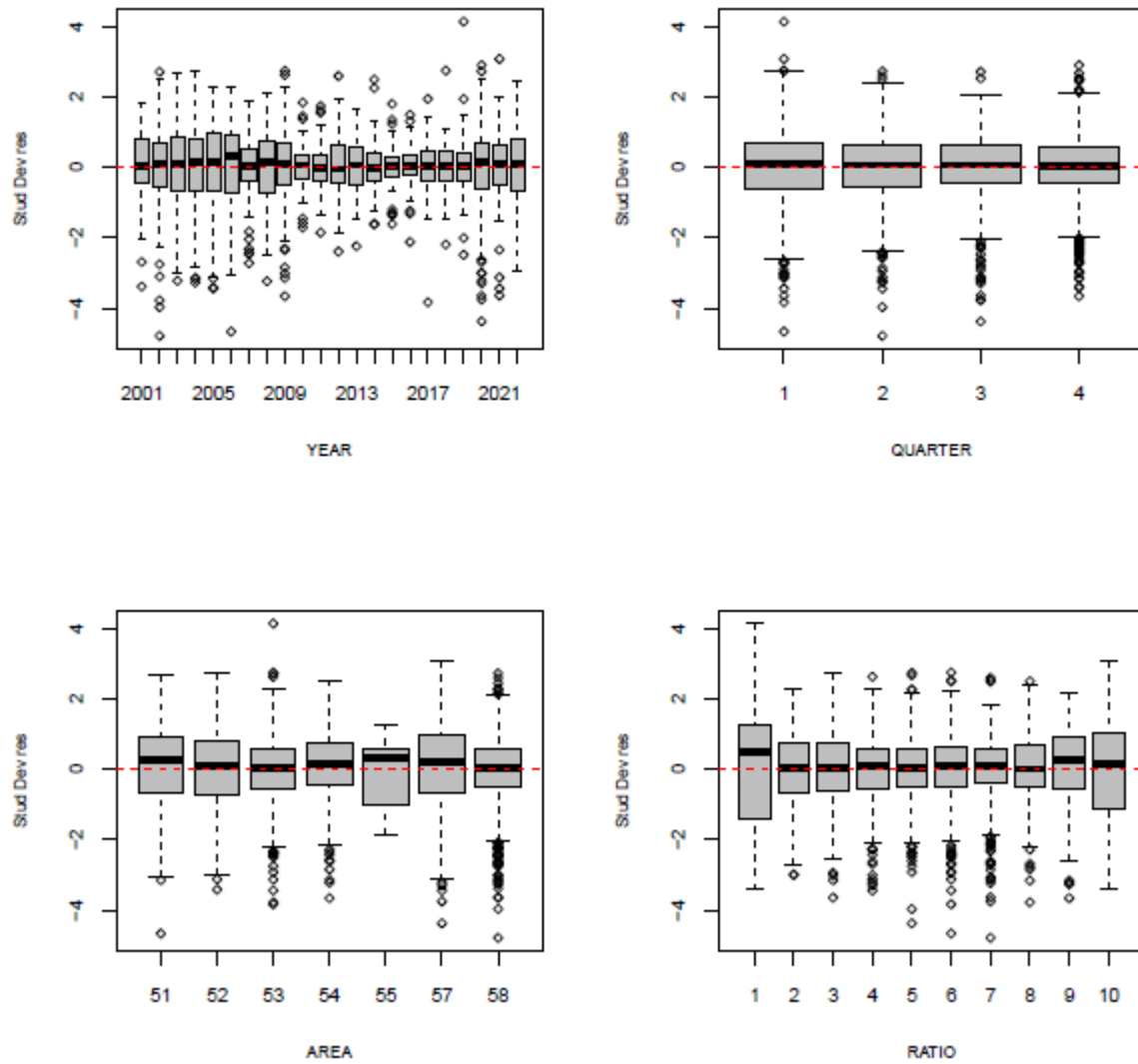
Figure 4. Box-plots of the standardized deviance residuals by explanatory variables obtained from the GLM base case in weight of shortfin mako for the Indian Ocean.
