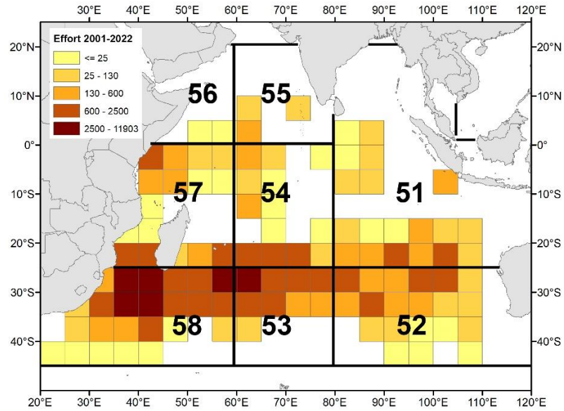
Figure 1. Area definition used for the GLM runs. Color scale represents the total nominal effort of this fleet (thousands of hooks) per 5x5 squares during the combined period 2001-2022.
