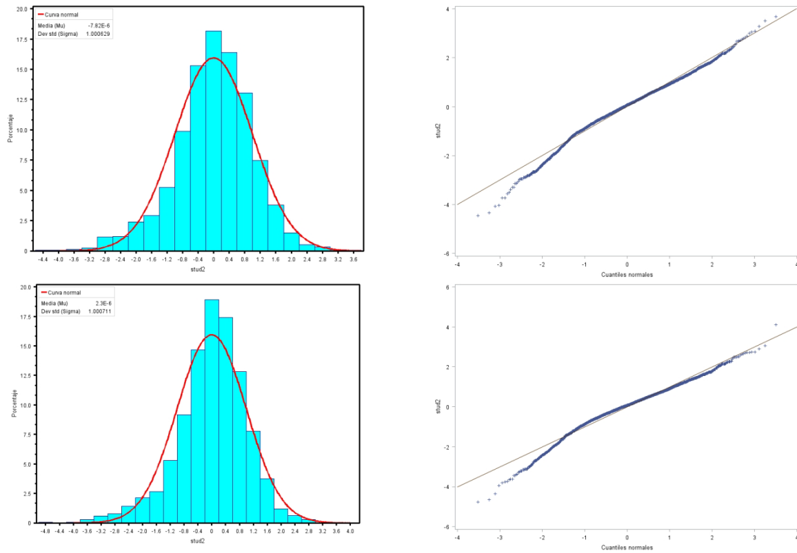
Figure 2. Diagnosis of the GLM runs for standardized CPUE in number of shortfin mako (upper) and in round weight (lower) for Indian Ocean: frequency distribution of the standardized residuals years combined (left panels) and normal probability qq-plot (right panels).
