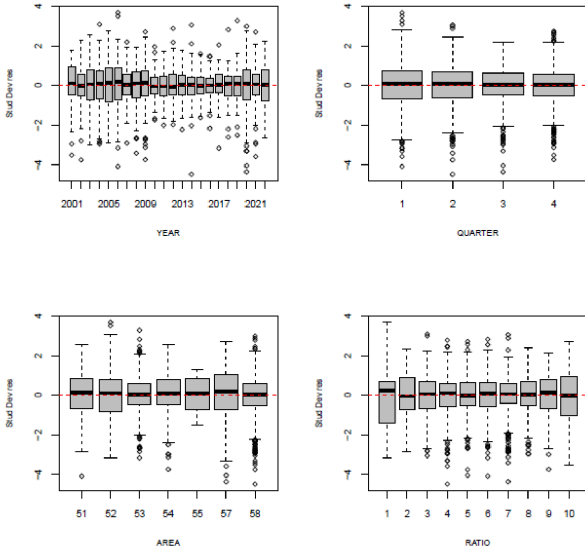
Figure 3. Box-plots of the standardized deviance residuals by explanatory variables obtained from the GLM base case in number of shortfin mako for the Indian Ocean.
