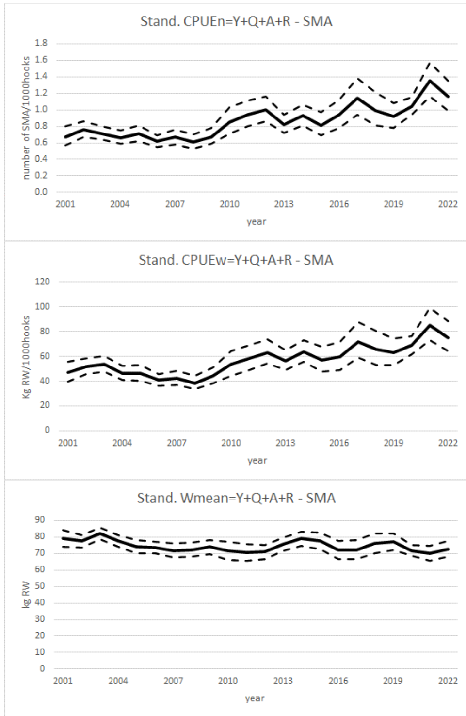
Figure 5. Standardized CPUEs per thousand hooks, in number of fish (upper), in kilograms round weight (middle) and standardized mean round weight in kilograms (lower) of shortfin mako and their respective confidence intervals (95%) observed in the Spanish surface longline fleet during the period analyzed (2001-2022) in the Indian Ocean.
